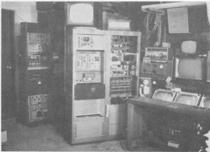
K4PDR's TV "studio" in Lutz, Fla. Lou Bellavia's control center, with one of his Ling Spectator cameras.
